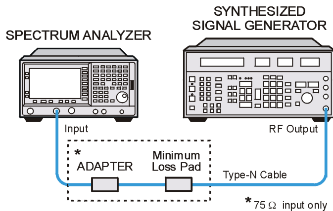
Figure 2-9 System-related Sidebands Test Setup
