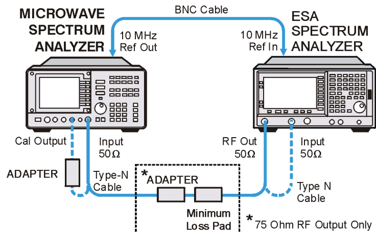
Figure 2-66 Harmonic Spurious Outputs Test Setup
