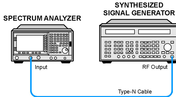
Figure 2-8 Noise Sidebands Test Setup
