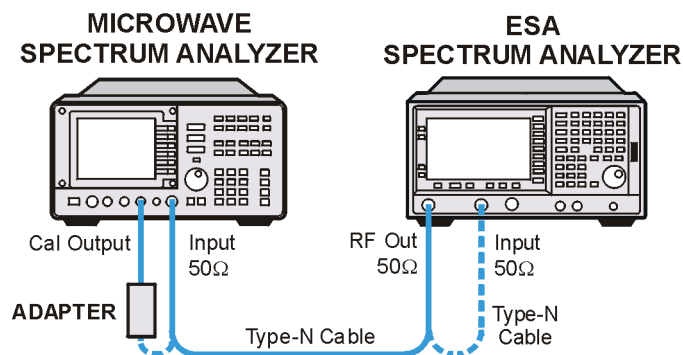
Figure 2-68 Non-Harmonic Spurious Outputs Test Setup
