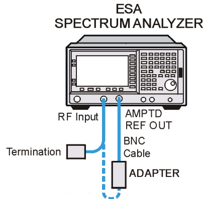
Figure 2-56 Displayed Average Noise Level Test Setup
