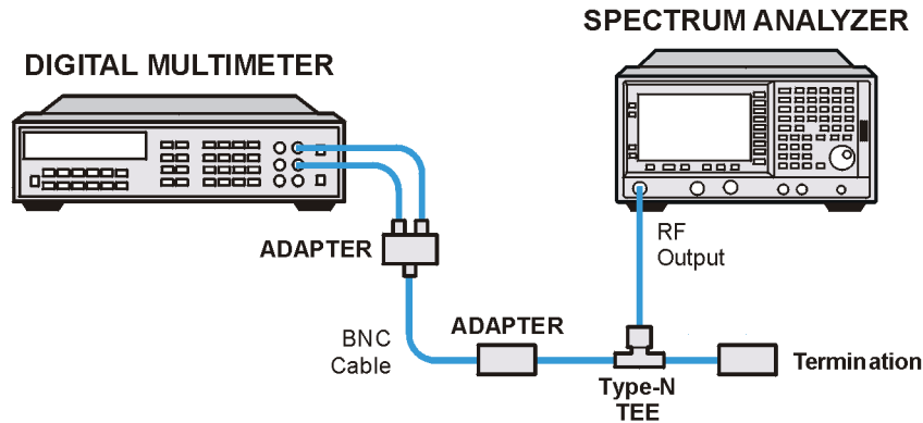
Figure 2-64 Tracking Generator Level Flatness Test Setup, \leq 100 kHz
