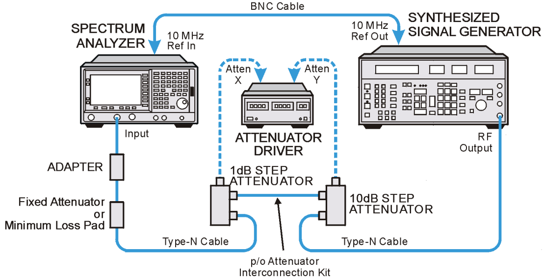
Figure 2-24 Amplitude Accuracy Test Setup
