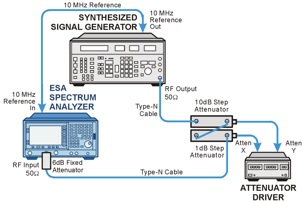
Figure 2-78 Amplitude Accuracy Test Setup
