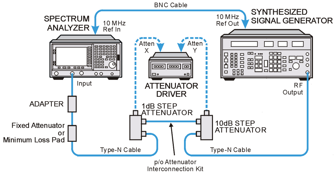
Figure 2-22 Amplitude Accuracy Test Setup
