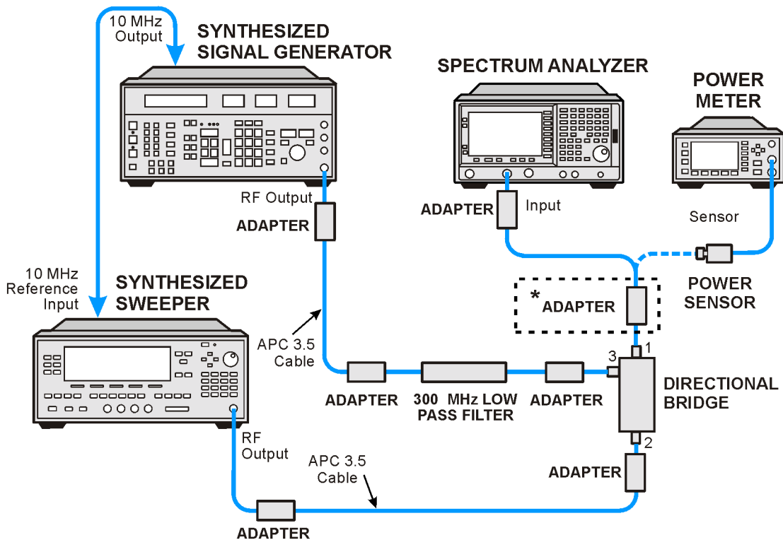
Figure 2-47 Third Order Intermodulation Distortion Test Setup
